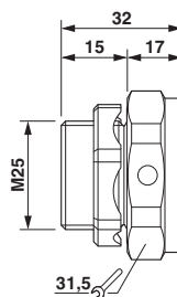
Dimensional drawing
